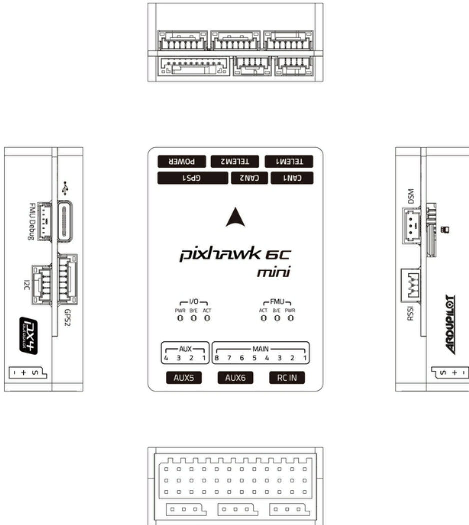
Pixhawk 6C Mini Model A (Current)
